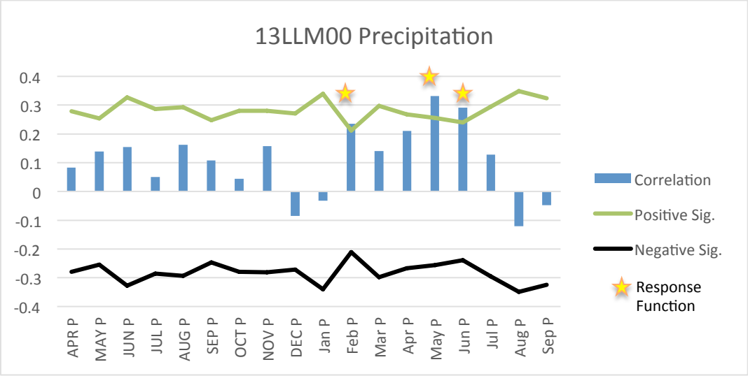
Figure 3: Results of the climate analysis comparing annual tree-ring growth to historical precipitation variables from Kelliher, SK.
