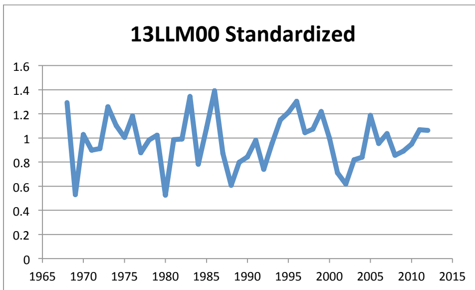
Figure 1: Master chronology for green ash at the Perry site. Standardized measurements of 1.00 indicate an average year of growth (in this case, associated with a raw ring-width of 2.03 mm), while any value above or below 1.00 indicate a year of growth that deviates from the average.
