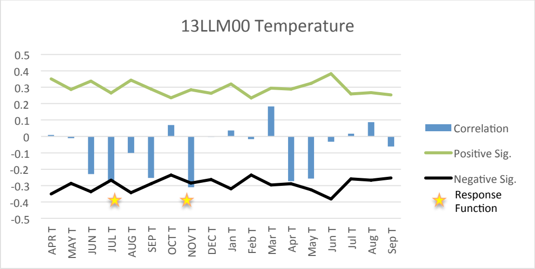
Figure 2: Results of the climate analysis comparing annual tree-ring growth to historical temperature variables from Kelliher, SK. The bars represent the degrees of correlation between the tree growth and the climate variable. The places where the bars cross the linear threshold are considered significantly correlated, marked by a star. The uppercase letters (ie., APR) label the previous years' variables.
