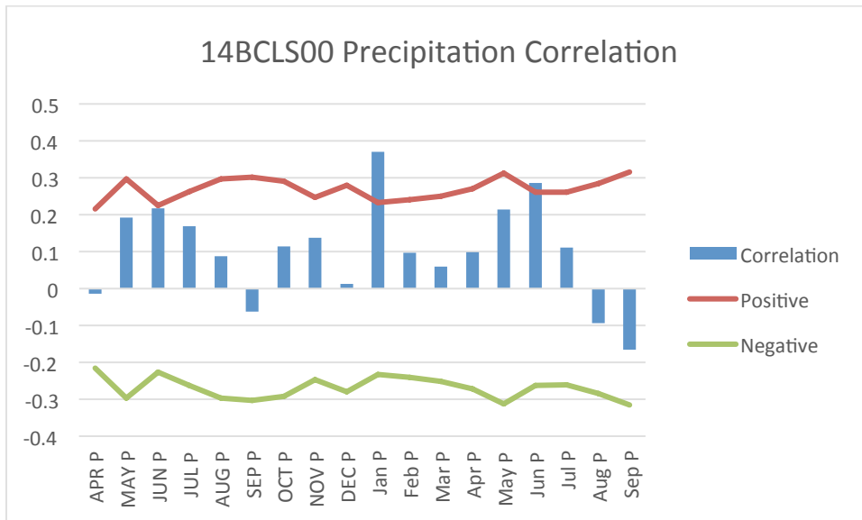
Figure 3: Results of the climate analysis comparing annual tree-ring growth to historical precipitation variables from Saskatoon, SK.
