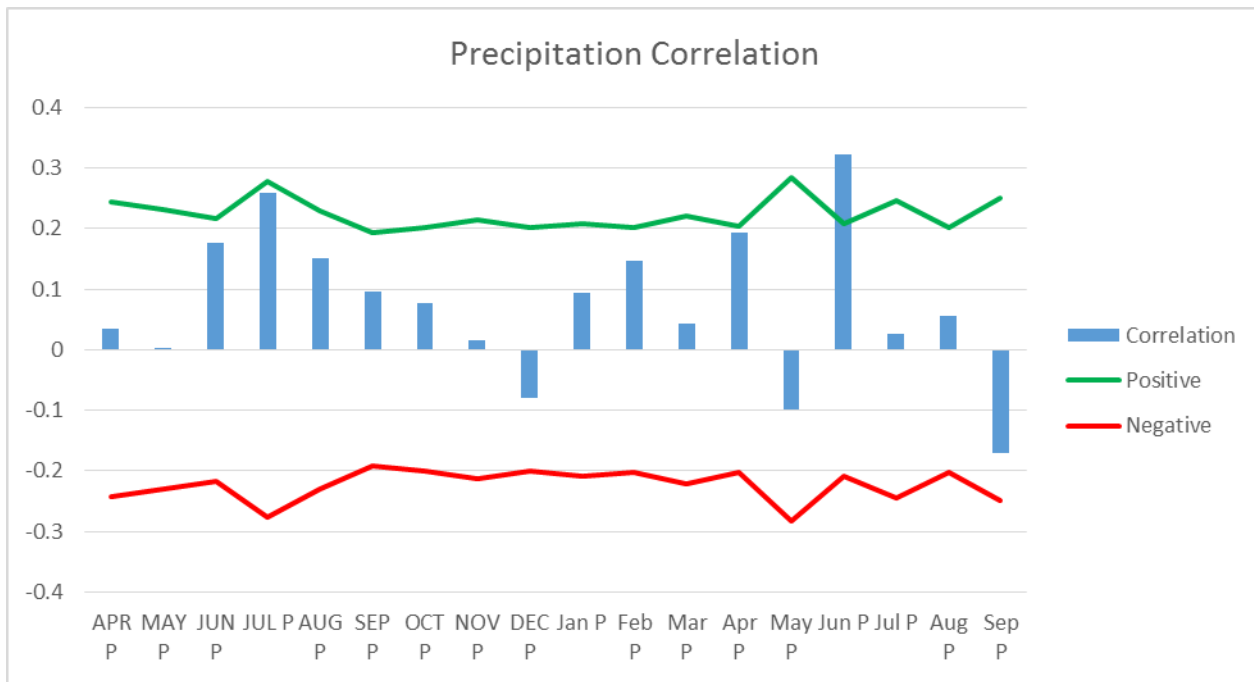
Figure 3: Results of the climate analysis comparing annual tree-ring growth to historical precipitation variables from Aneroid, SK.
