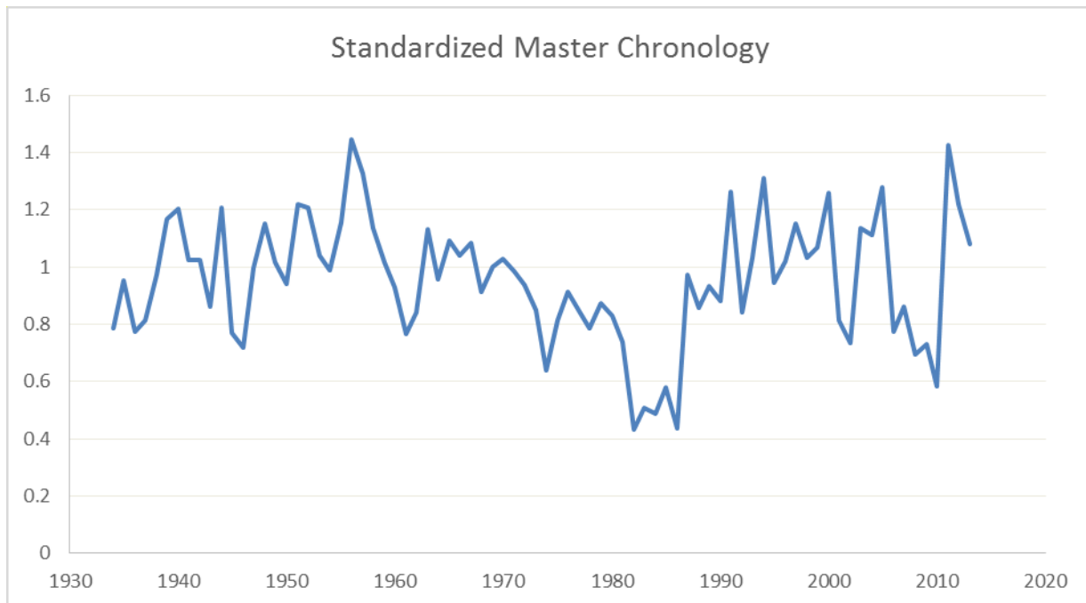
Figure 1: Master chronology for hybrid poplar at the Iffy Nipper site. Standardized measurements of 1.00 indicate an average year of growth (in this case, associated with a raw ring-width of 3.72 mm), while any value above or below 1.00 indicate a year of growth that deviates from the average.
