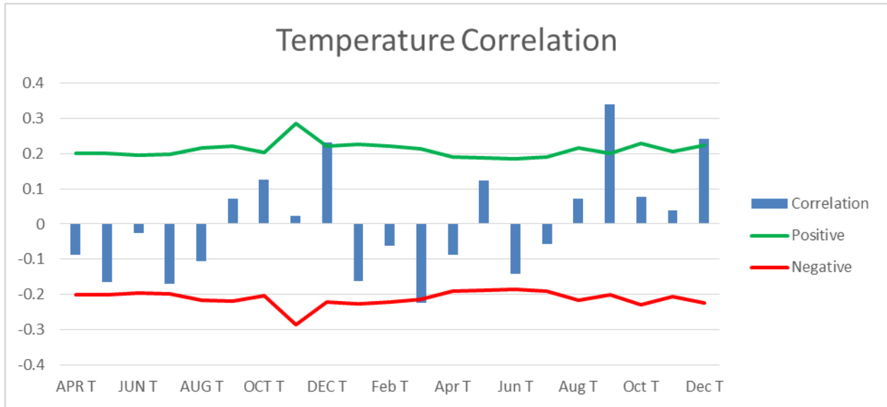
Figure 2: Results of the climate analysis comparing annual tree-ring growth to historical temperature variables from Aneroid, SK. The bars represent the degrees of correlation between the tree growth and the climate variable. The places where the bars cross the linear threshold are considered significantly correlated. The uppercase letters (ie., APR) label the previous years' variables.
