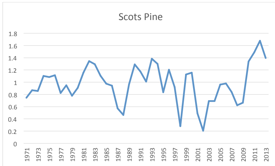
Figure 1: Master chronology for Scots pine at the Sparks Farm site. Standardized measurements of 1.00 indicate an average year of growth (in this case, associated with a raw ring-width of 2.62 mm), while any value above or below 1.00 indicate a year of growth that deviates from the average.
