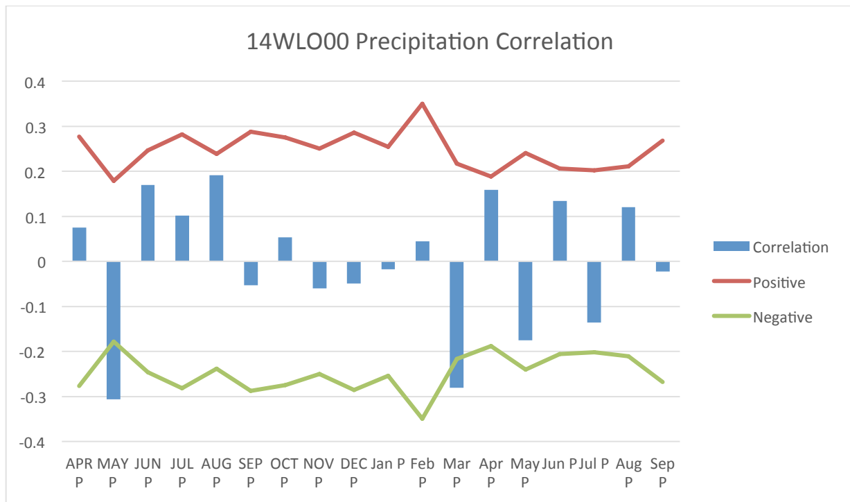
Figure 3: Results of the climate analysis comparing annual tree-ring growth to historical precipitation variables from Poplar River, SK.
