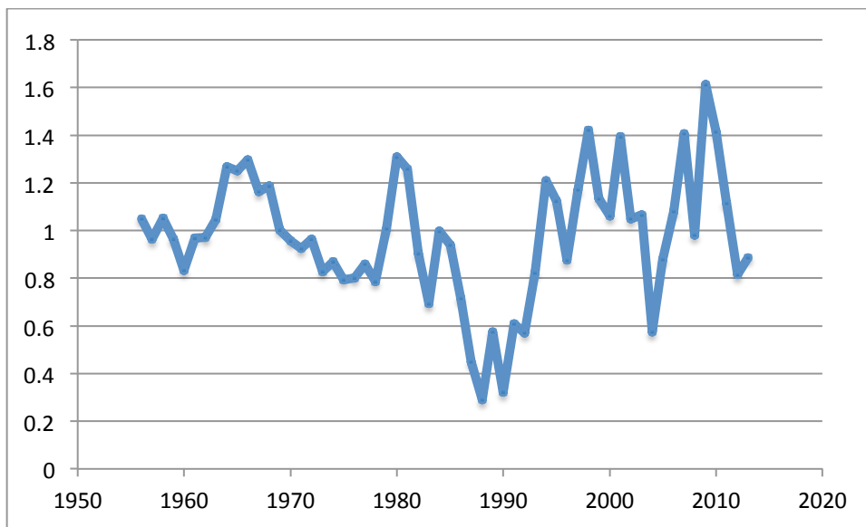
Figure 1: Master chronology for Manitoba maple at the Philippon Farm site. Standardized measurements of 1.00 indicate an average year of growth (in this case, associated with a raw ring-width of 1.82 mm), while any value above or below 1.00 indicate a year of growth that deviates from the average.
