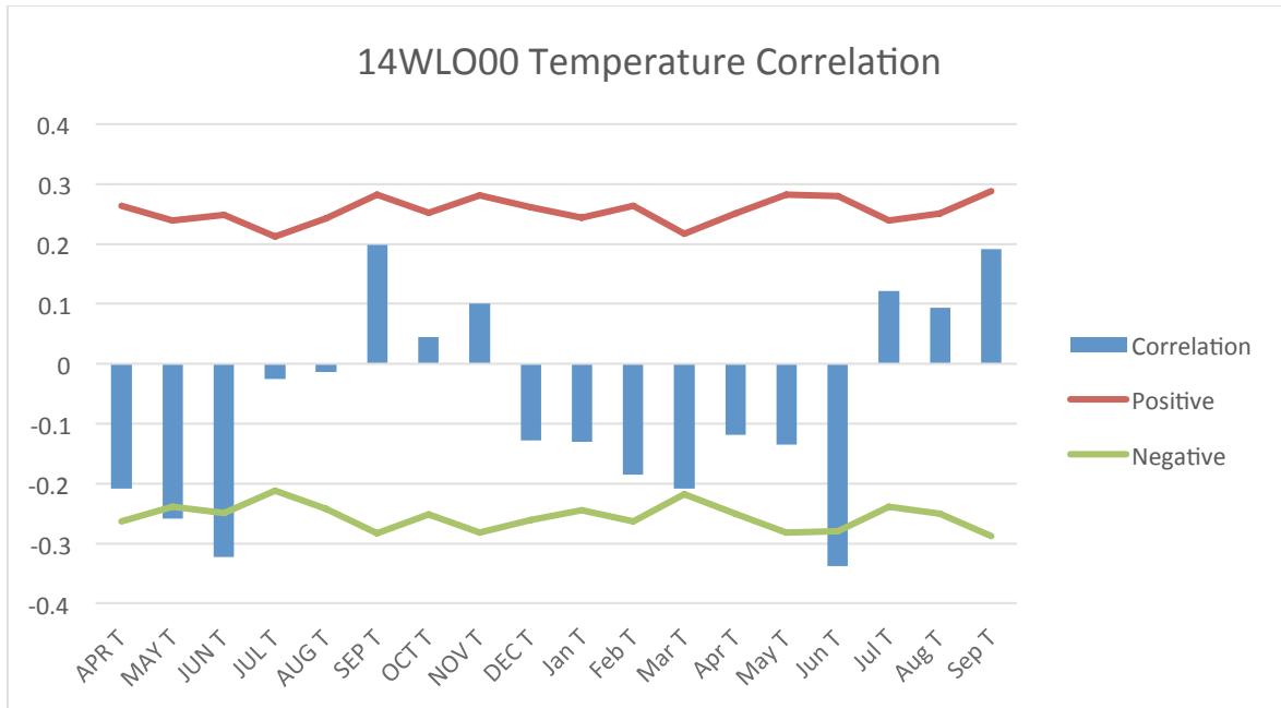
Figure 2: Results of the climate analysis comparing annual tree-ring growth to historical temperature variables from Poplar River, SK. The bars represent the degrees of correlation between the tree growth and the climate variable. The places where the bars cross the linear threshold are considered significantly correlated. The uppercase letters (ie., APR) label the previous years' variables.
